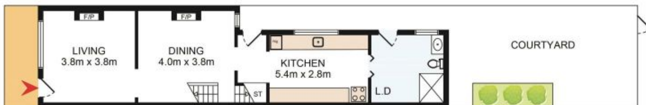
GROUND FLOOR
